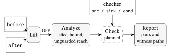
Figure 4: Pipeline of AUTHDIFF. Two versions are lifted to GFP, analyzed, and compared; Report emits the newly unconditioned pairs and their witness paths. Check (planned) will evaluate a checker specification over the guarded slice.
